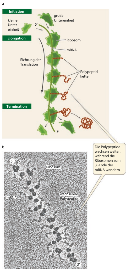
▣ Abb. 2.6 Translation [39]
